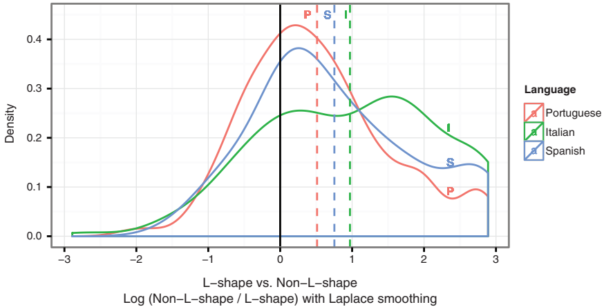
Figure 2: Density of Response Preference by Participant – Portuguese (Red), Italian (Green), Spanish (Blue); the solid line indicates the neutral response preference, and the dashed lines indicate the mean of the log ratio for each language.
