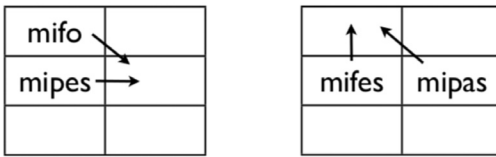
Figure 1: Schematic representation of the I \rightarrow S condition (left) and S \rightarrow I condition (right).
