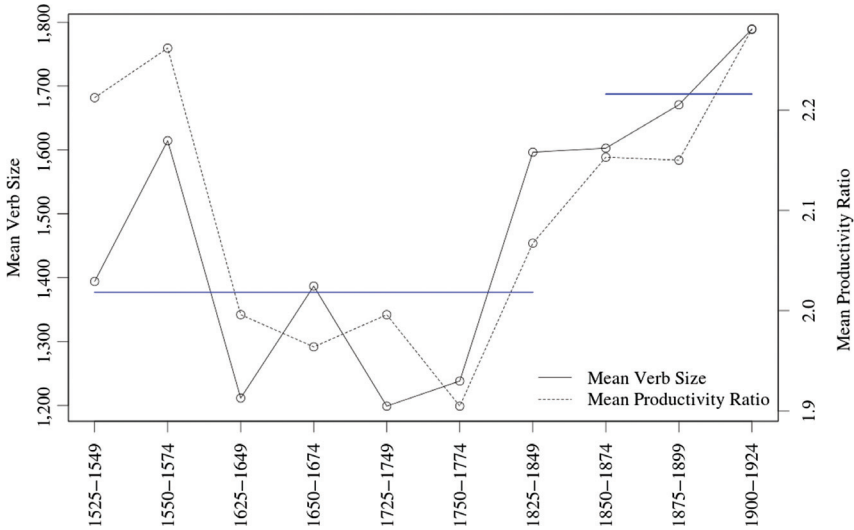
Figure 5: Temporal trends of verb vocabulary size and productivity with changepoint analysis; Language: Portuguese, Corpus: Colonia, Size: 5.1 million words, Epoch volume: 114,173 words (for verb vocabulary size estimation) and 1,252 verbs (for productivity estimation).
